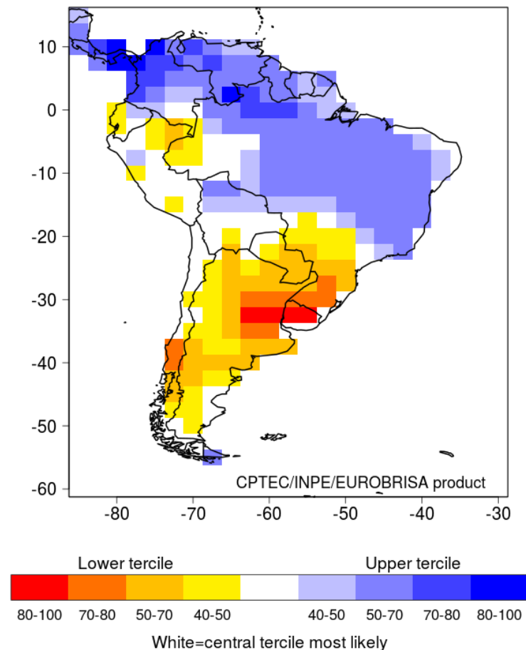
Integrated: Prob. of most likely precip. tercile (%) Issued: Sep 2021 Valid for OND 2021
