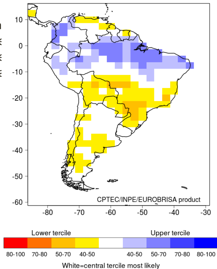
Integrated: Prob. of most likely precip. tercile (%) Issued: Apr 2021 Valid for MJJ 2021
