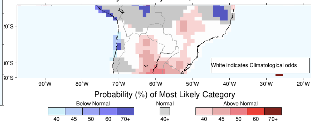
IRI Multi-Model Probability Forecast for Temperature for December–January–February 2022, Issued November 2021
