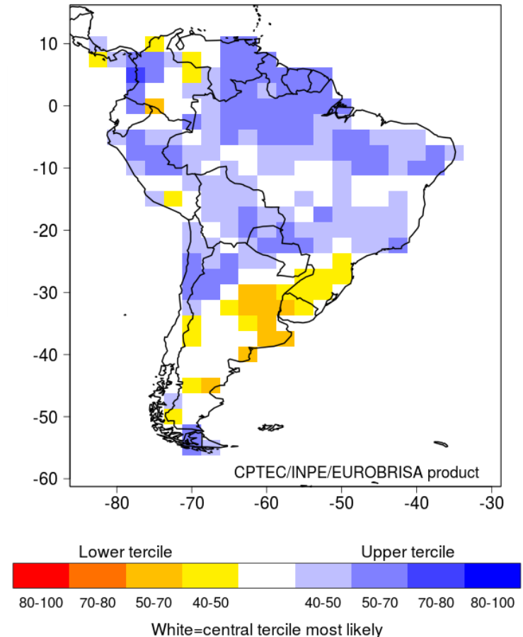
Integrated: Prob. of most likely precip. tercile (%) Issued: Jan 2021 Valid for FMA 2021
