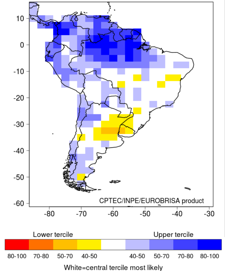
Integrated: Prob. of most likely precip. tercile (%) Issued: Dec 2020 Valid for JFM 2021
