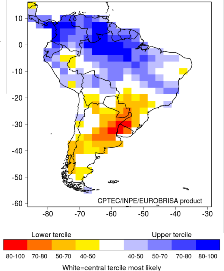
Integrated: Prob. of most likely precip. tercile (%) Issued: Oct 2020 Valid for NDJ 2020
