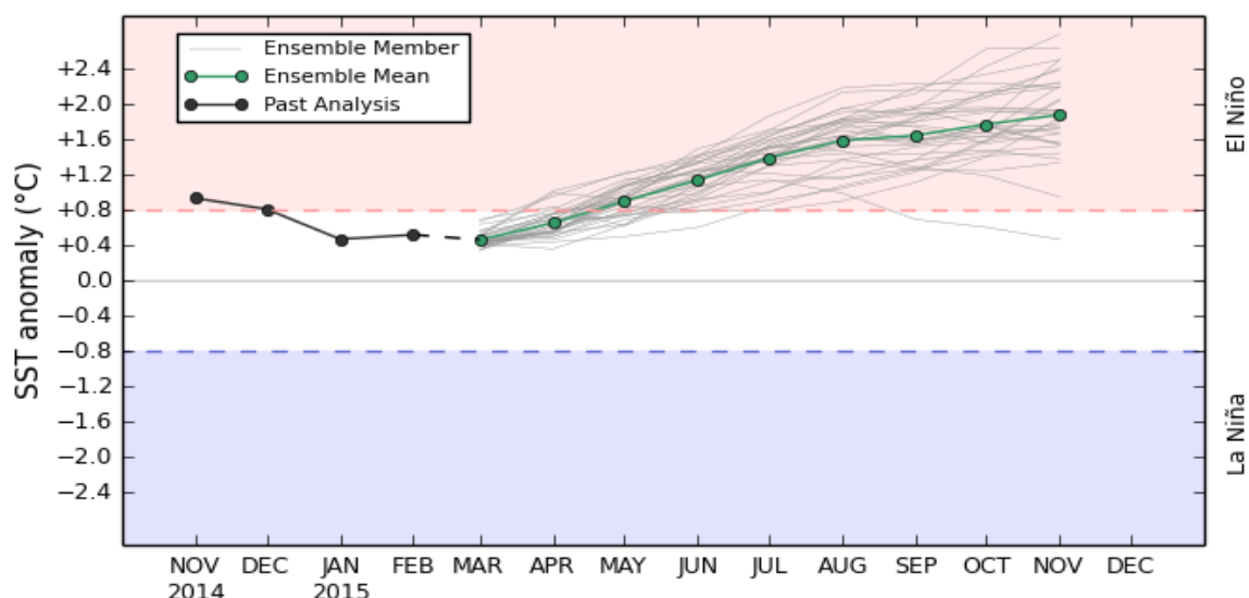
POAMA monthly mean NINO34 - Forecast Start: 1 MAR 2015
