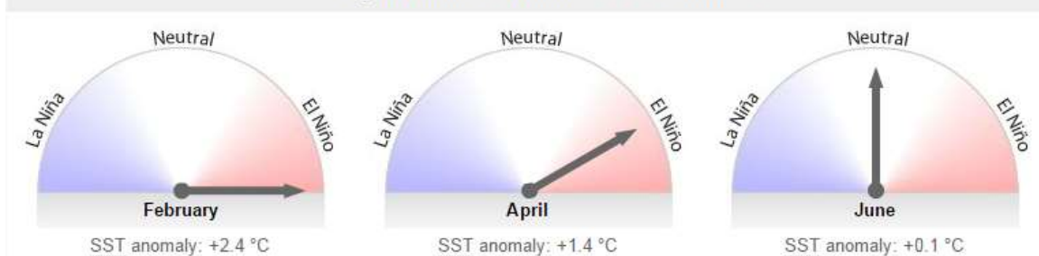
Average of international model outlooks for NINO3.4
