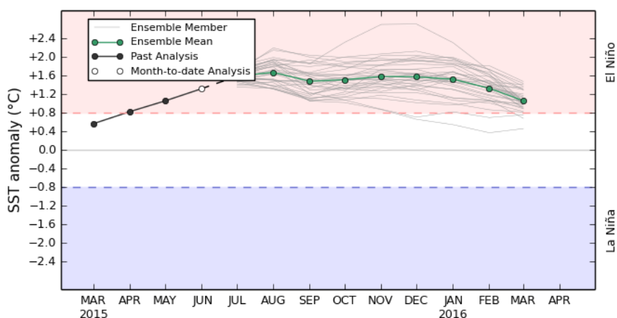
POAMA monthly mean NINO34 - Forecast Start: 21 JUN 2015
