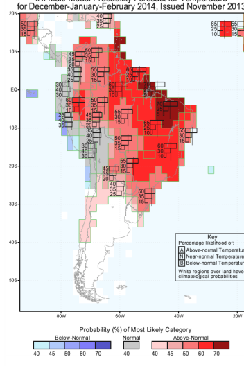
IRI Multi-Model Probability Forecast for Temperature for December-January-February 2014, issued November 2013
