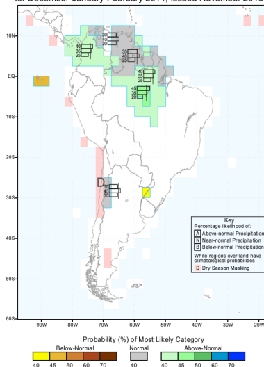
IRI Multi-Model Probability Forecast for Precipitation for December-January-February 2014, issued November 2013
