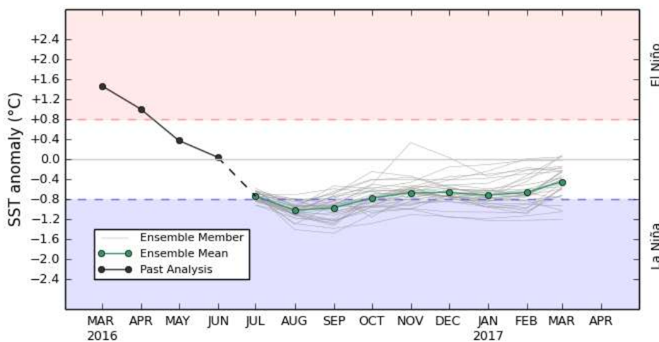
POAMA monthly mean NINO34 - Forecast Start: 3 JUL 2016
